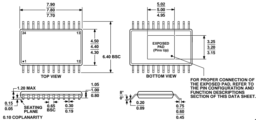
Figure 81. 24-Lead Thin Shrink Small Outline Package, Exposed Pad [TSSOP_EP] (RE-24)
