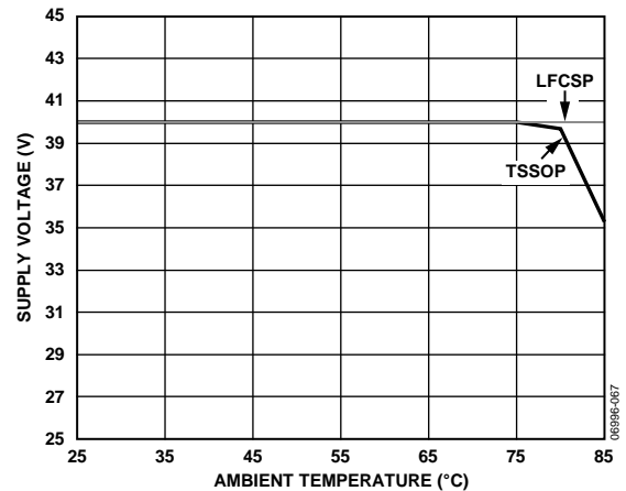
Figure 78. Maximum Supply Voltage vs. Ambient Temperature
