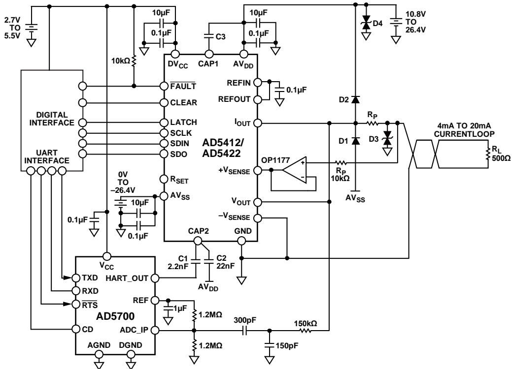
Figure 79. AD5412/AD5422 in HART Configuration
