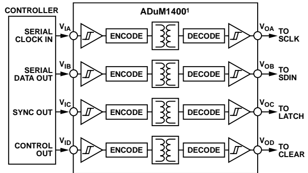
Figure 76. Isolated Interface
