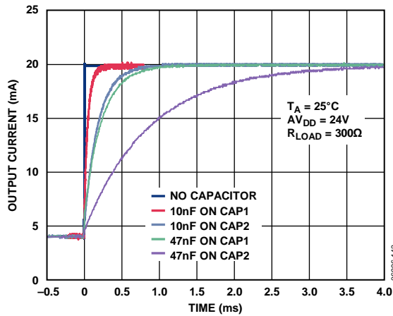
Figure 72. Slew Controlled 4 mA to 20 mA Output Current Step Using
