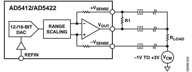
Figure 65. Voltage Output
