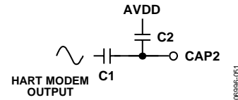
Figure 68. Coupling HART Signal
