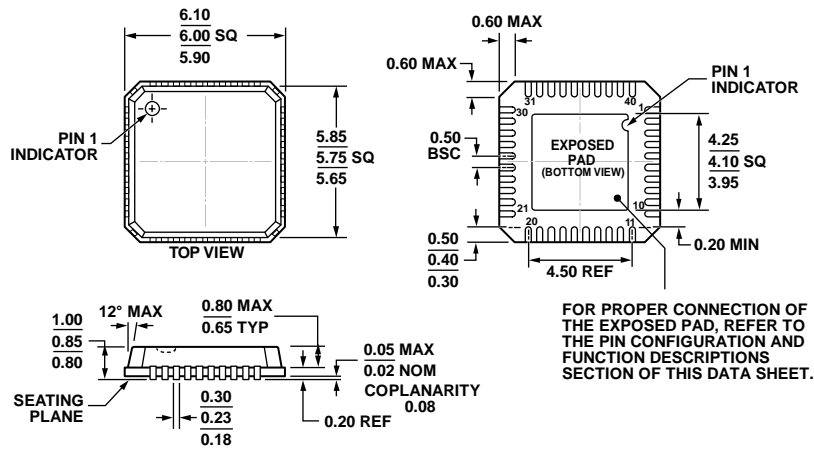
Figure 82. 40-Lead Lead Frame Chip Scale Package [LFCS_P_VQ] 6 mm x 6 mm Body, Very Thin Quad (CP-40-1)
