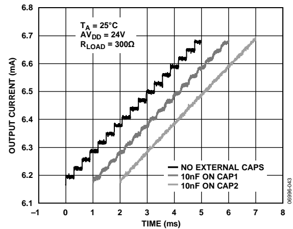
Figure 73. Smoothing Out the Steps Caused by the Digital Slew Rate Control Feature
