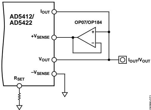
Figure 74. Isolated Interface
