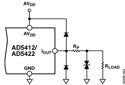
Figure 75. Output Transient Voltage Protection
