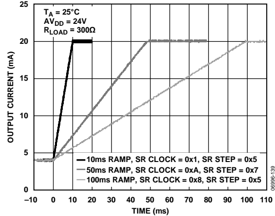
Figure 69. Output Current Slewing Under Control of the Digital Slew Rate Control Feature
