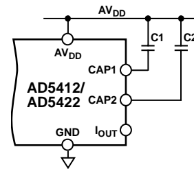
Figure 70. I_{OUT} Filtering Capacitors
