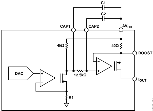
Figure 71. I_{OUT} Filter Circuitry
