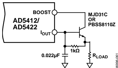
Figure 67. External Boost Configuration
