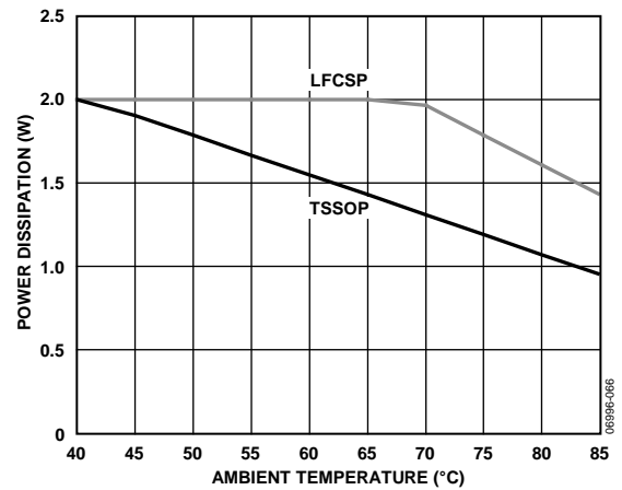
Figure 77. Maximum Power Dissipation vs. Ambient Temperature
